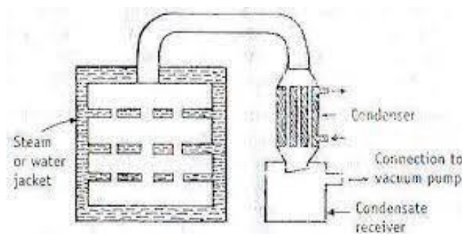
Figure 14-7. Vacuum dryer.
